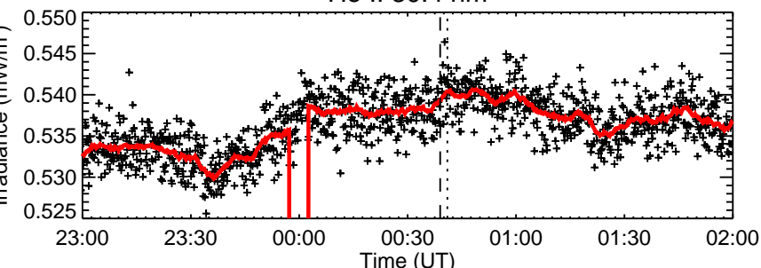
RHESSI Quicklook
