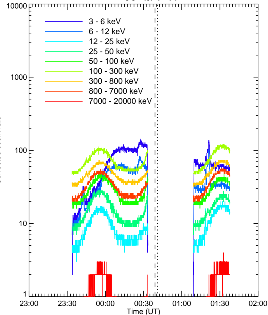
RHESSI Quicklook
