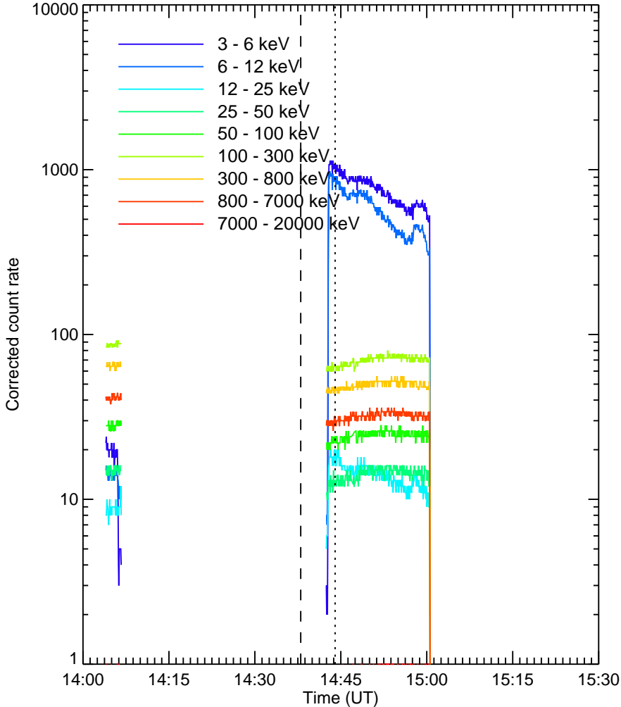
RHESSI Quicklook
