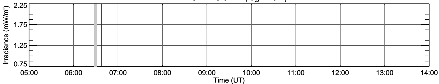
EVE O IV 55.4 nm (log T=5.2)
