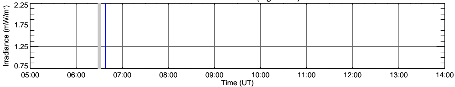
EVE O V 63.0 nm (log T=5.4)
