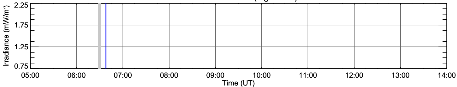
EVE O IV 79.0 nm (log T=5.2)
