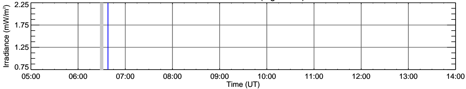
EVE O III 60.0 nm (log T=4.9)
