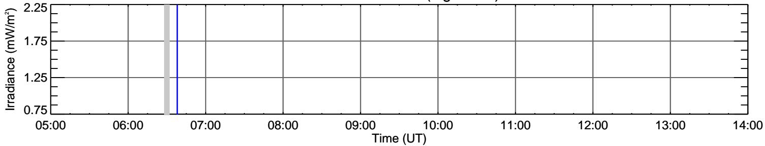
EVE O III 52.6 nm (log T=4.9)
