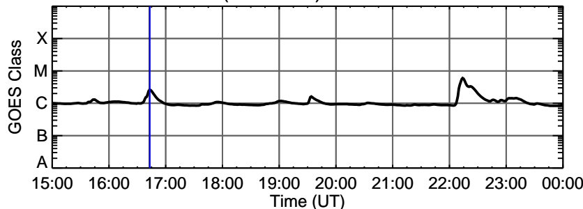
12-Dec-2013 (DOY 346) C2.6 @ 16:43:00 UT
