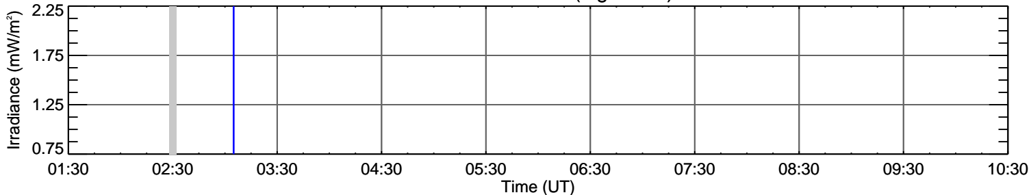
EVE O III 52.6 nm (log T=4.9)
