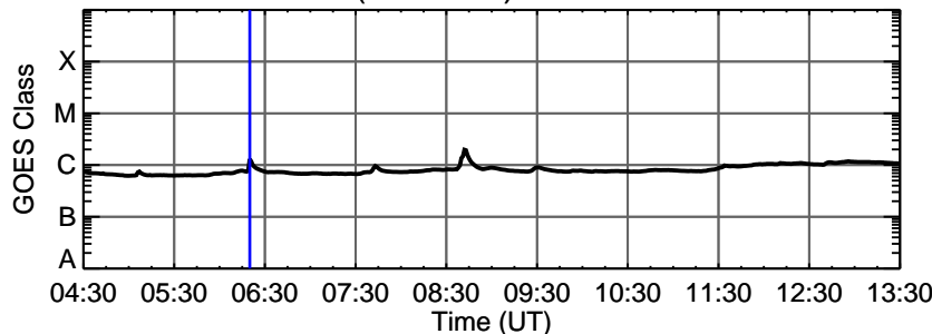
16-Dec-2013 (DOY 350) C1.3 @ 06:20:00 UT
