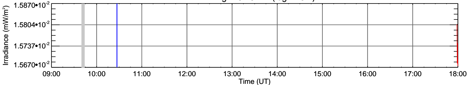
EVE Mg X 62.5 nm (log T=6.1)
