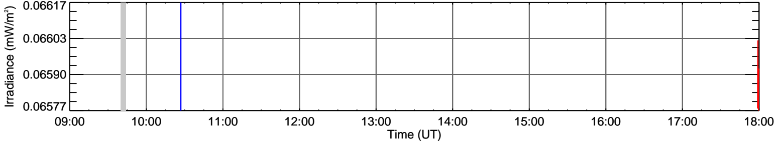
EVE H I 102.6 nm (log T=3.8)
