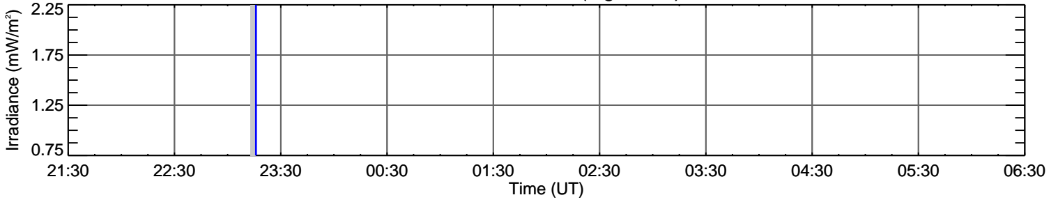
EVE He I 58.4 nm (log T=4.2)
