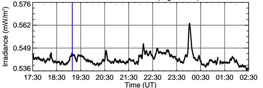
ESP 30.4 nm
