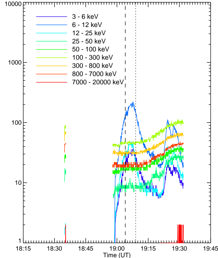
RHessi Quicklook
