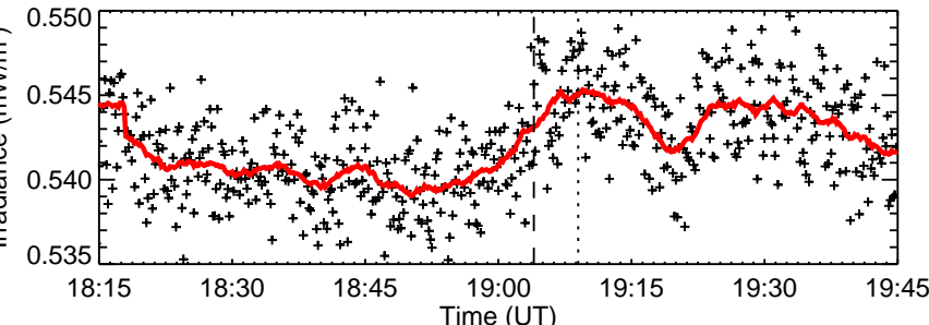
RHessi Quicklook
