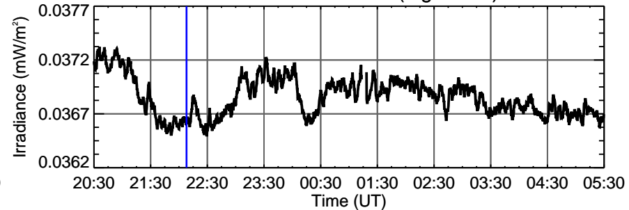
EVE Fe XII 19.5 nm (log T=6.1)
