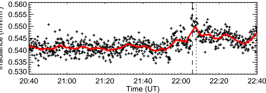
RHESSI Quicklook
