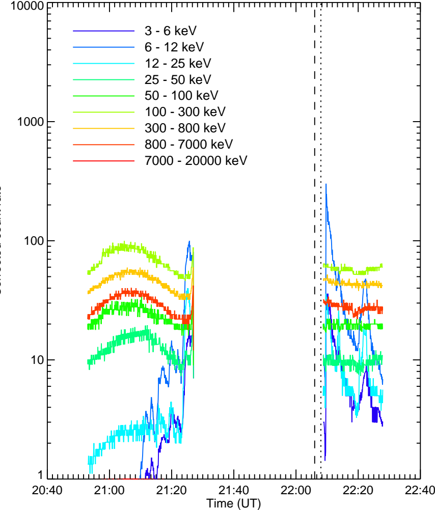
RHESSI Quicklook
