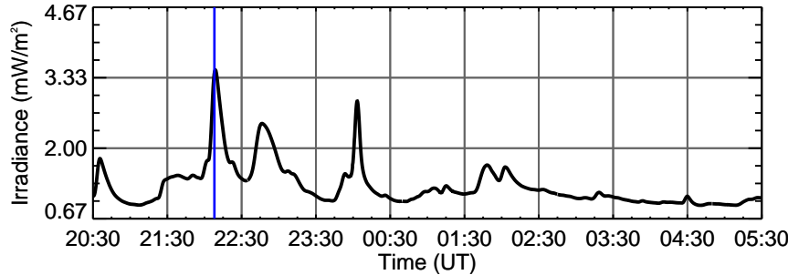
EVE Fe XX 13.3 nm (log T=7.0)
