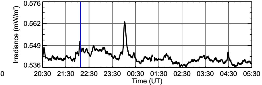
ESP 30.4 nm
