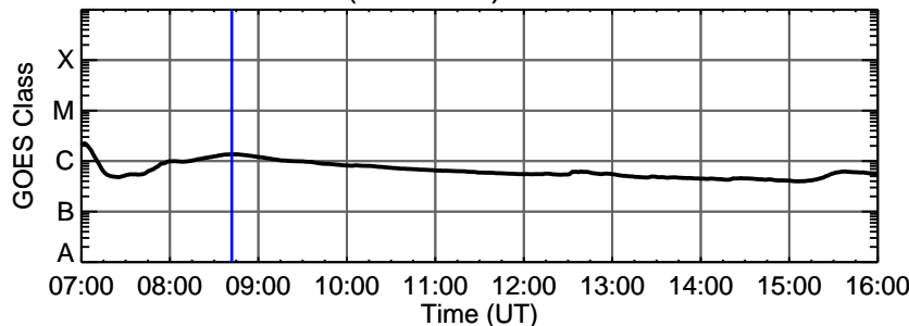
26-Dec-2013 (DOY 360) C1.3 @ 08:42:00 UT
