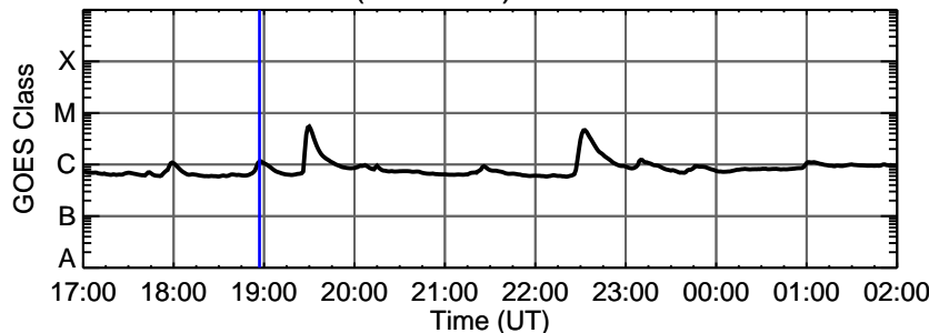
29-Dec-2013 (DOY 363) C1.1 @ 18:57:00 UT
