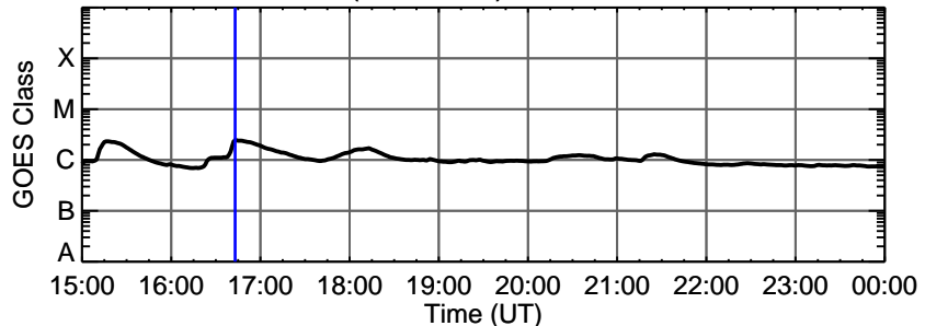
30-Dec-2013 (DOY 364) C2.4 @ 16:43:00 UT
