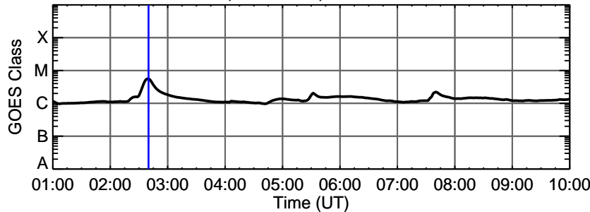
31-Dec-2013 (DOY 365) C5.6 @ 02:40:00 UT
