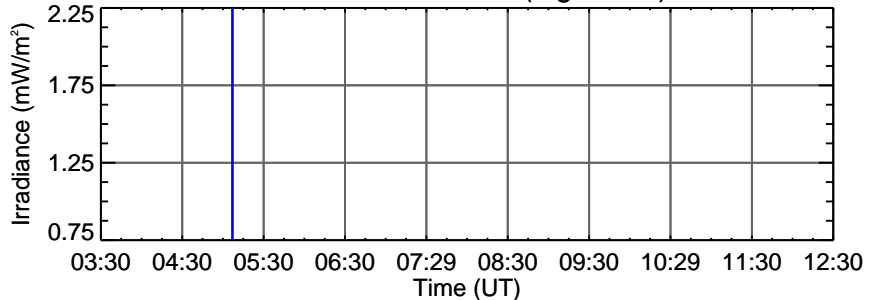
ESP 30.4 nm
