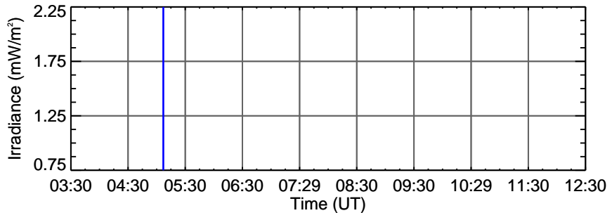
ESP 30.4 nm
