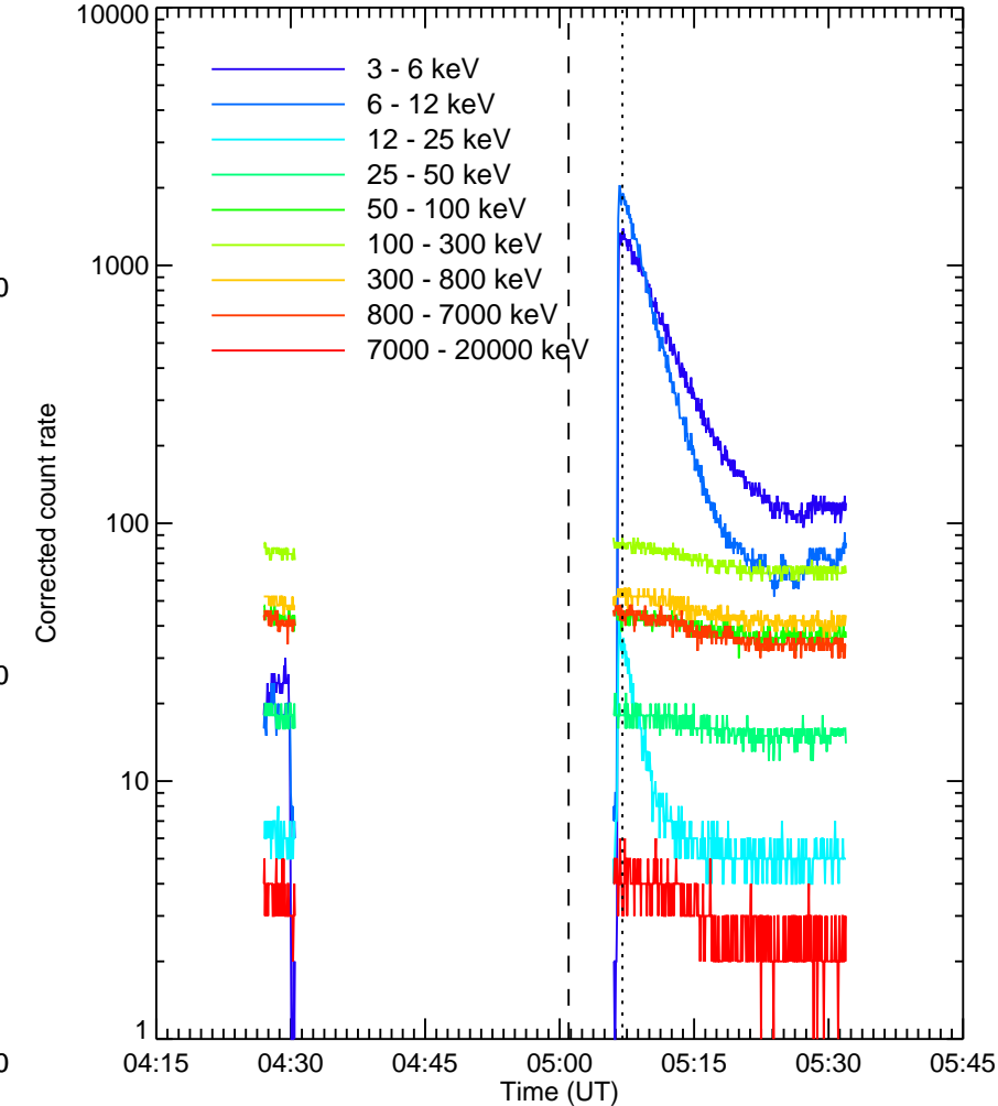
RHESSEI Quicklook
