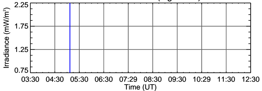
EVE Fe IX 17.1 nm (log T=5.8)
