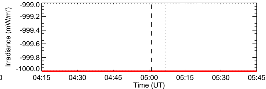
RHESSEI Quicklook
