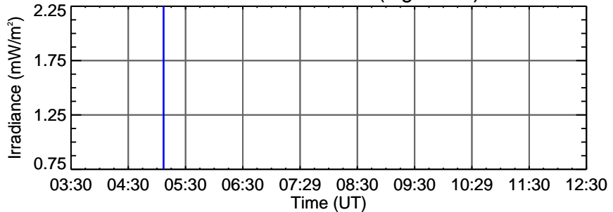
EVE Fe XII 19.5 nm (log T=6.1)
