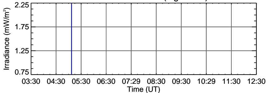
EVE Fe X 17.7 nm (log T=6.0)
