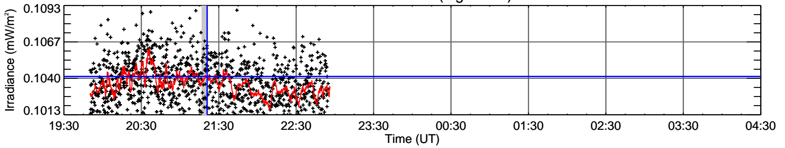
EVE H I 97.3 nm (log T=3.8)
