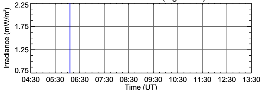
EVE Fe XVI 33.5 nm (log T=6.4)
