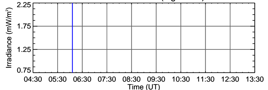
ESP 30.4 nm
