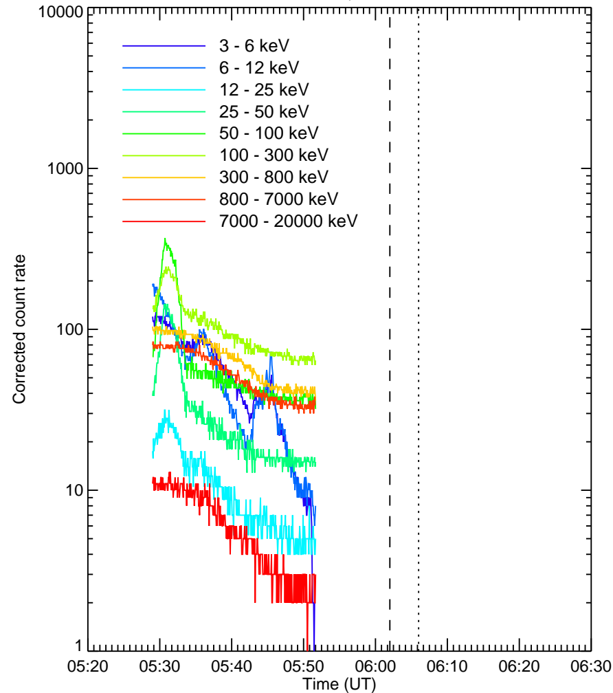
RHESSI Quicklook
