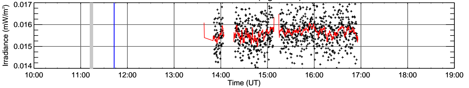
EVE He I 53.7 nm (log T=3.8)
