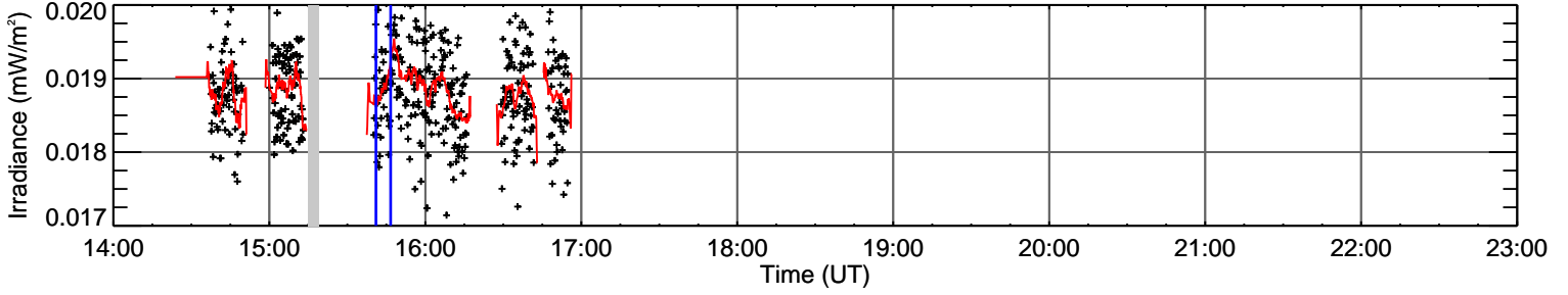
EVE H I 95.0 nm (log T=3.8)
