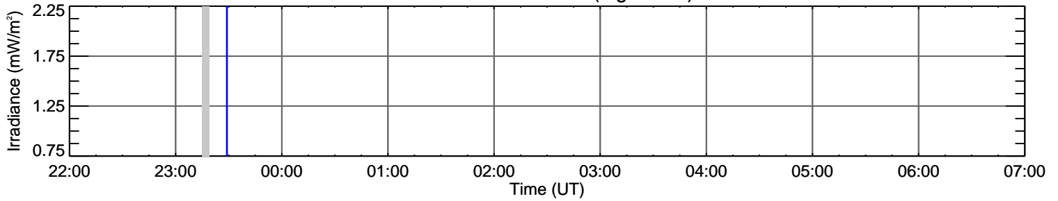
EVE Si XII 49.9 nm (log T=6.3)
