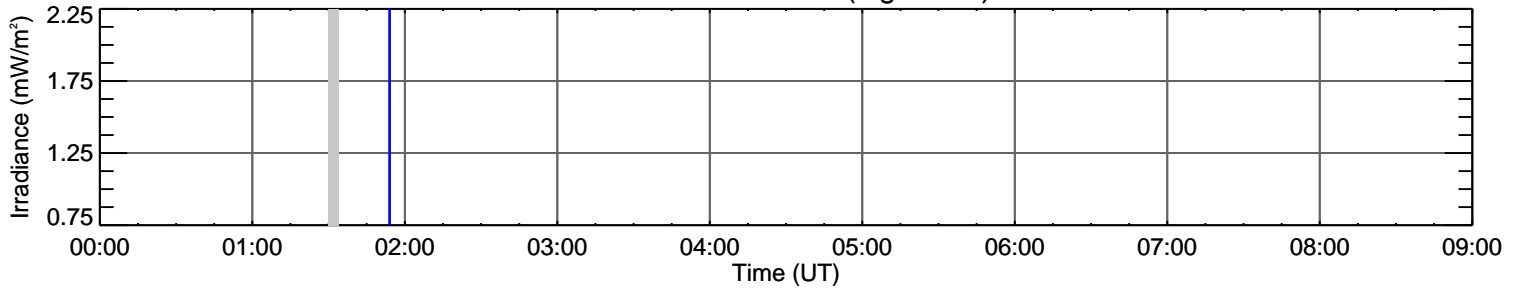
EVE Ne VII 46.5 nm (log T=5.7)
