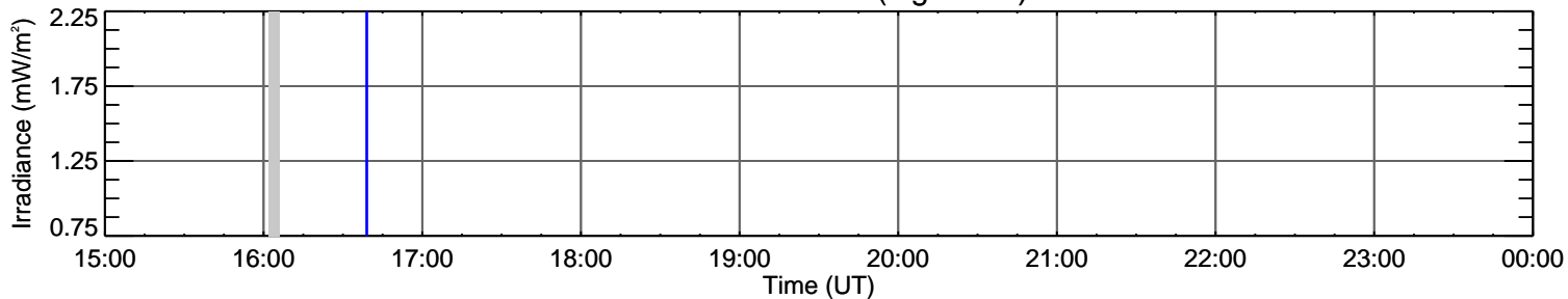
EVE He II 30.4 nm (log T=4.7)
