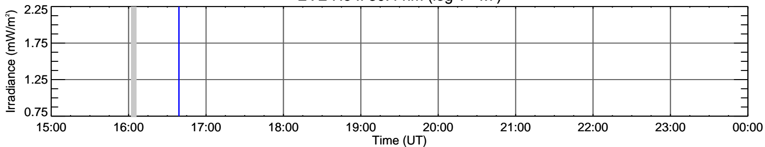
EVE O II 83.6 nm (log T=4.5)
