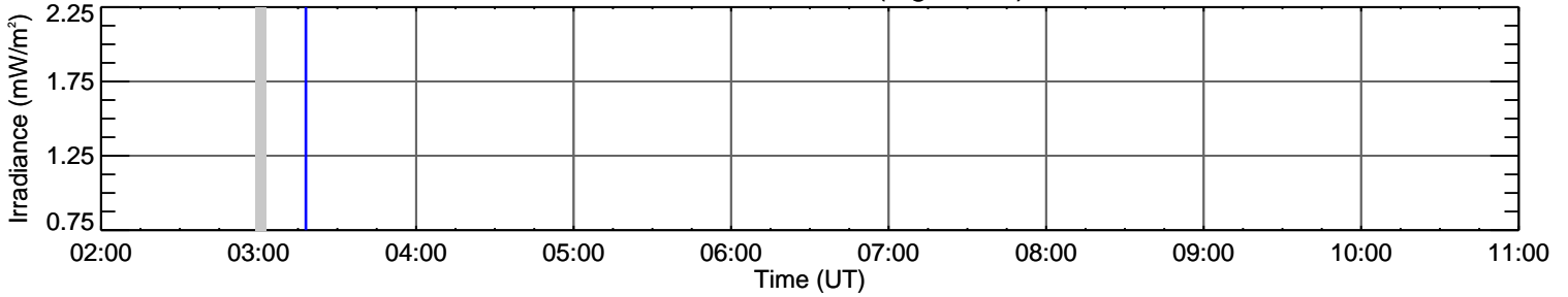
EVE Mg X 61.0 nm (log T=6.1)
