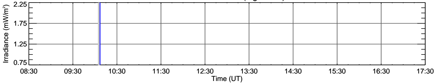
EVE O II 83.6 nm (log T=4.5)
