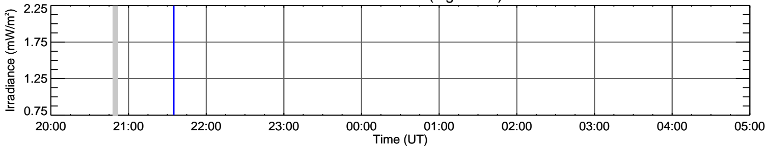
EVE Ne VIII 77.0 nm (log T=5.8)
