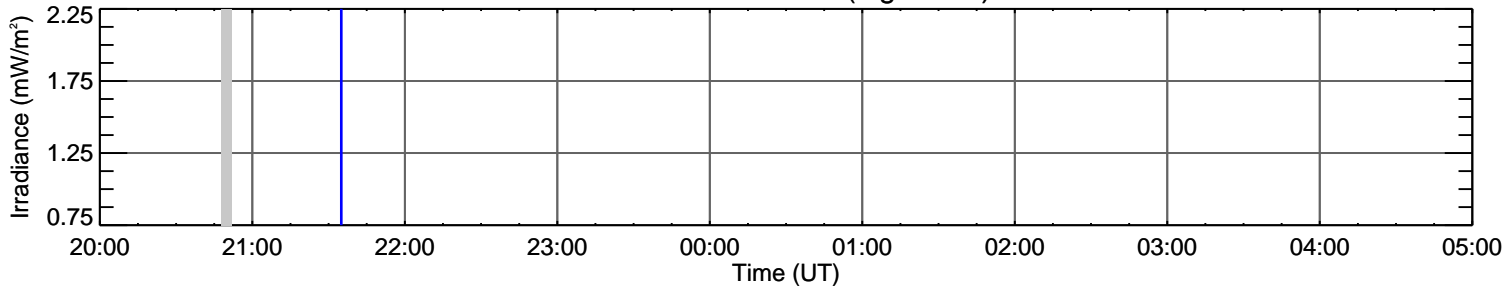
EVE Ne VII 46.5 nm (log T=5.7)
