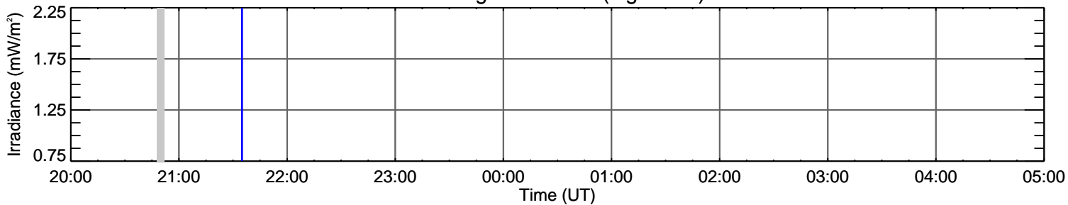
EVE Fe X 17.7 nm (log T=6.0)
