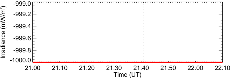
RHESSI Quicklook
