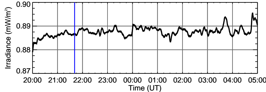
ESP 30.4 nm
