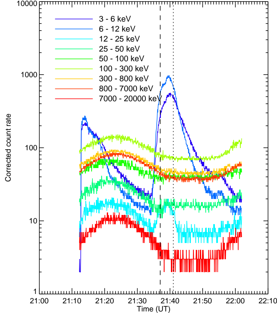
RHESSI Quicklook
