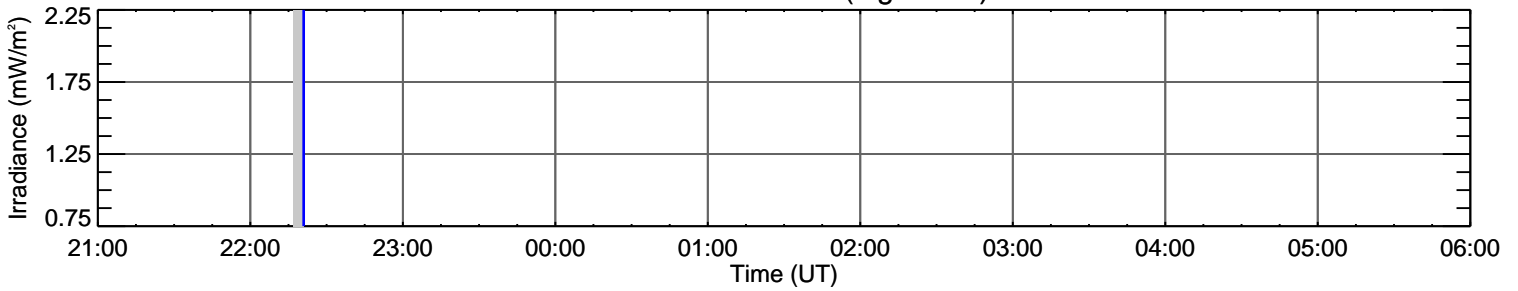
EVE Si XII 52.1 nm (log T=6.3)
