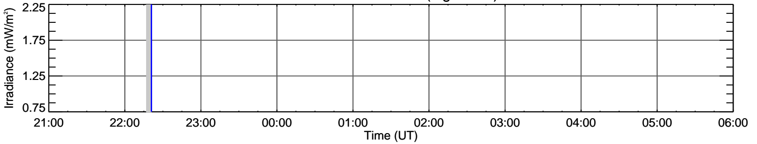
EVE Fe IX 17.1 nm (log T=5.8)
