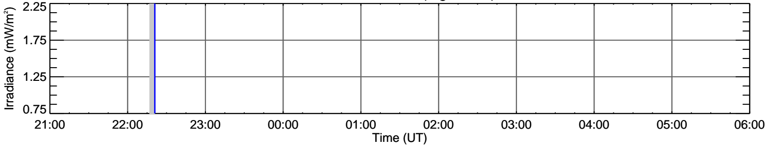
EVE H I 95.0 nm (log T=3.8)
