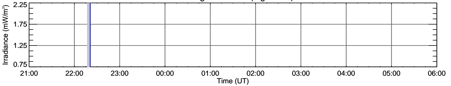
EVE Mg X 62.5 nm (log T=6.1)
