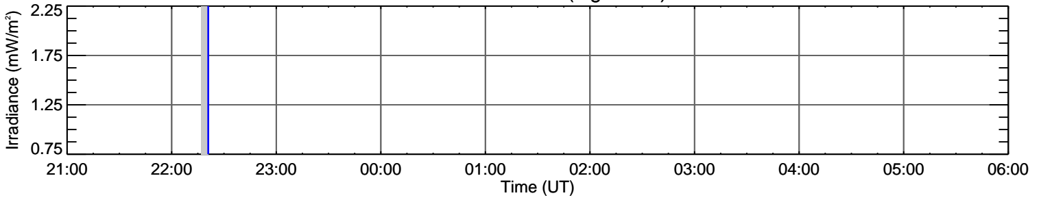
EVE He I 53.7 nm (log T=3.8)
