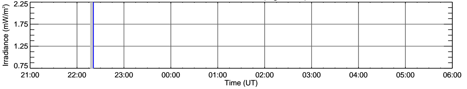
EVE Fe XVI 33.5 nm (log T=6.4)
