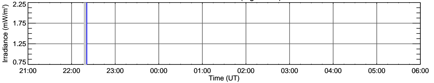
EVE O II 83.6 nm (log T=4.5)
