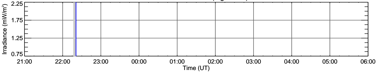
EVE Fe XVI 36.1 nm (log T=6.4)
