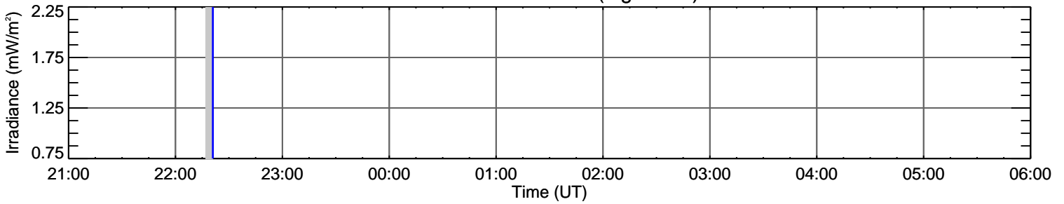
EVE Fe VIII 13.1 nm (log T=5.6)
