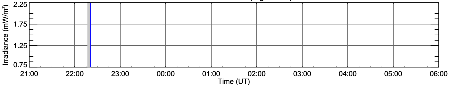
EVE H I 97.3 nm (log T=3.8)
