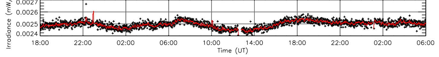
O VI 103.19 nm (log T=5.47)
