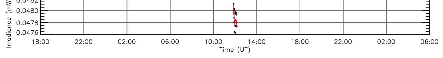
O IV 79.02 nm (log T=5.19)
