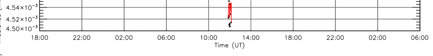
O III 52.58 nm (log T=4.92)
