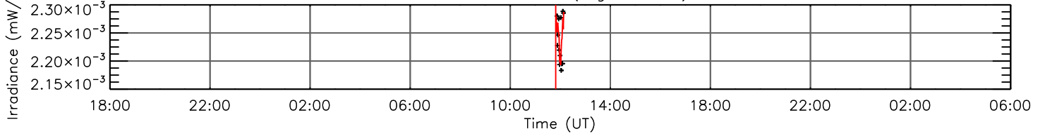
He I 58.43 nm (log T=4.16)
