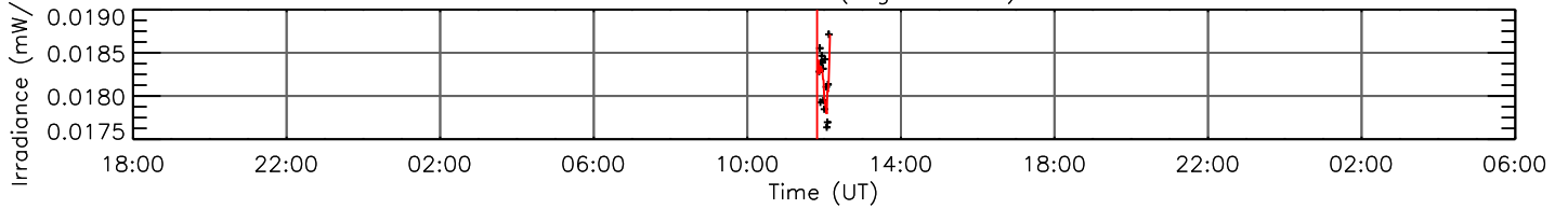
H I 97.25 nm (log T=3.84)
