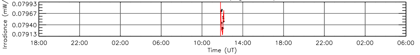
H I 97.25 nm (log T=3.84)
