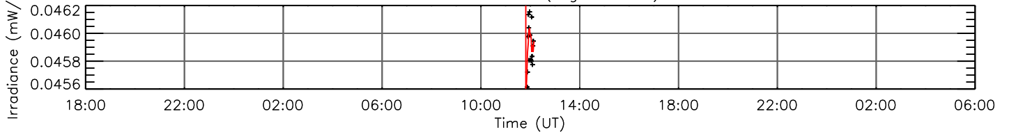
H I 102.57 nm (log T=3.84)
