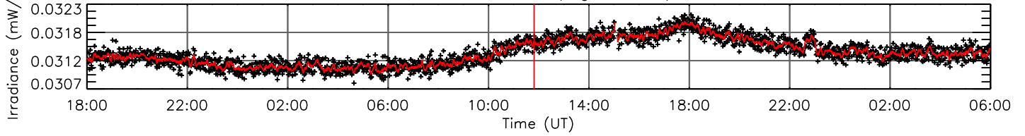
He II 30.38 nm (log T=4.70)
