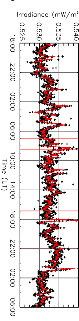
He II 30.38 nm (log T=4.70)
