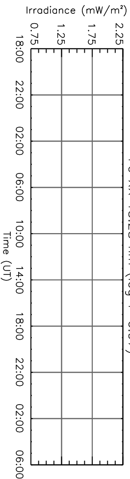
Fe XVIII 9.39 nm (log T=6.81)
