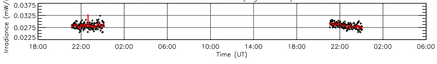
Fe XVI 33.54 nm (log T=6.43)
