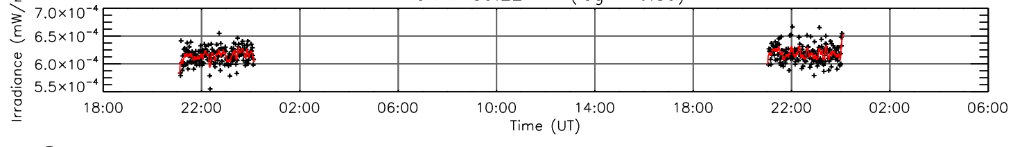
Fe XVIII 9.39 nm (log T=6.81)
