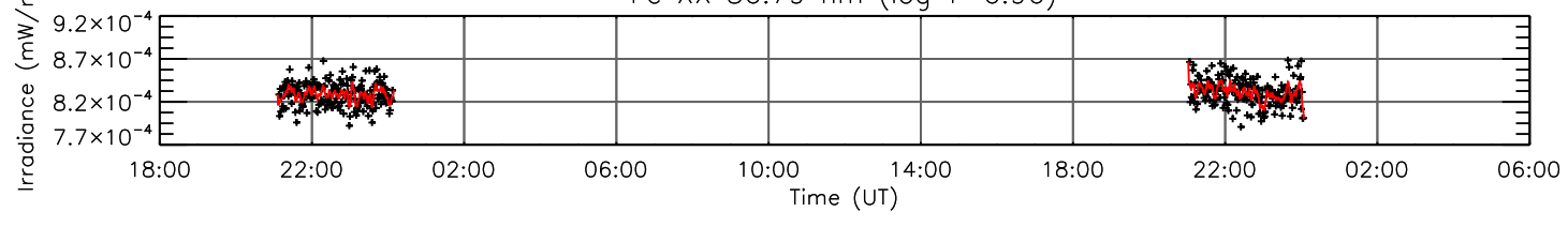
Fe XIX 59.22 nm (log T=6.89)
