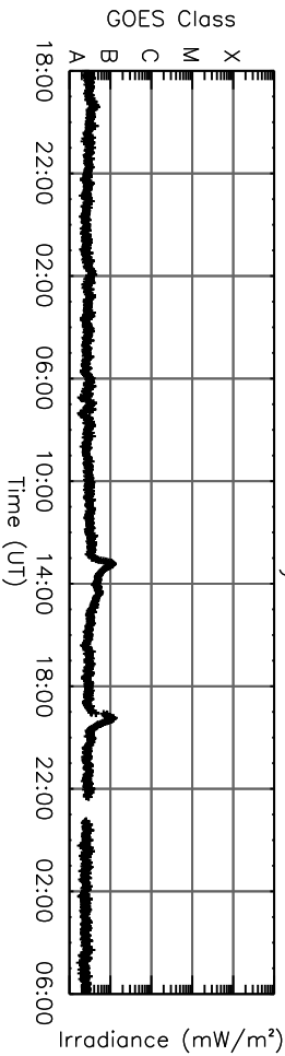
GOES X-ray Flux
