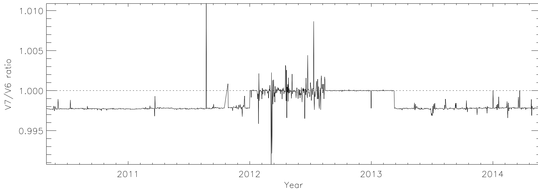
Fe X 17.724
