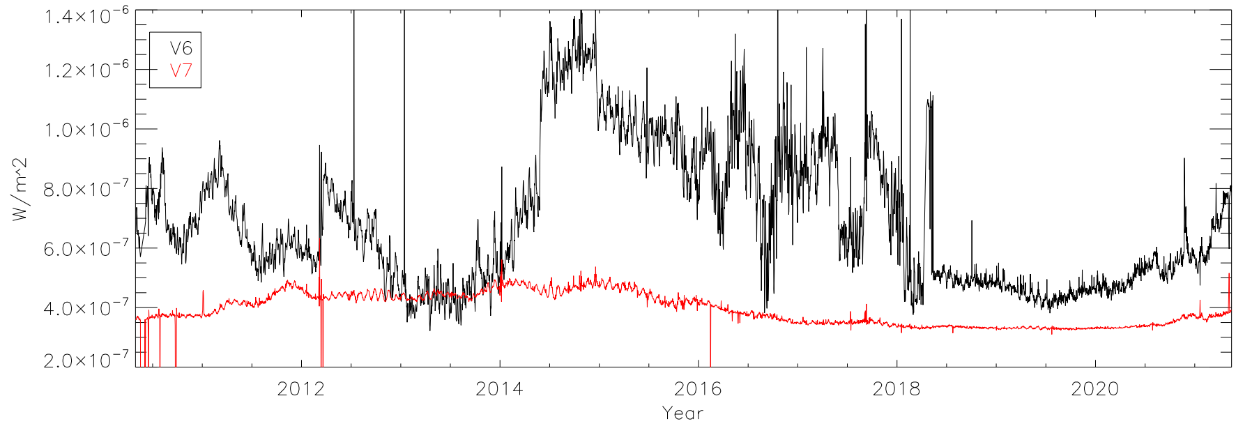
Fe XX 72.156
