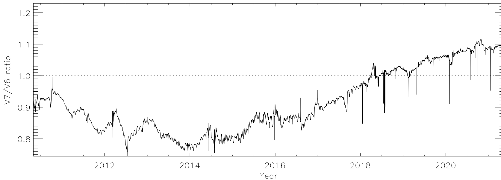
He I 53.700
