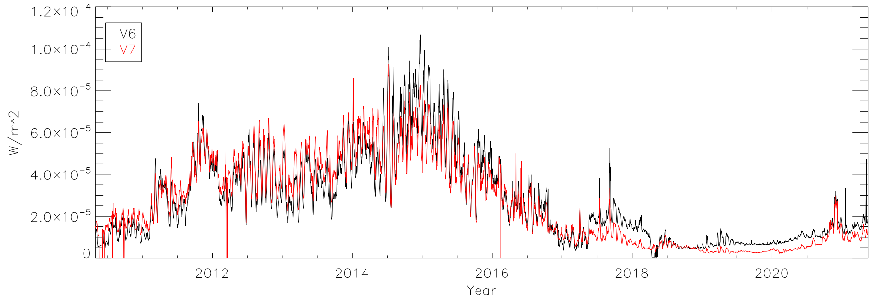
Fe XVI 33.541
