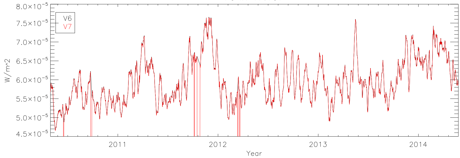
Fe IX 17.107
