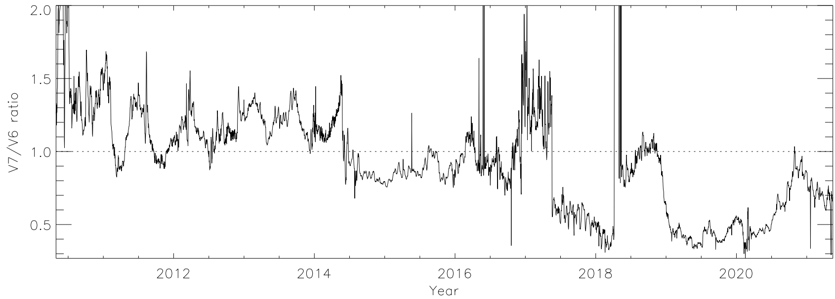
Fe XVI 33.541
