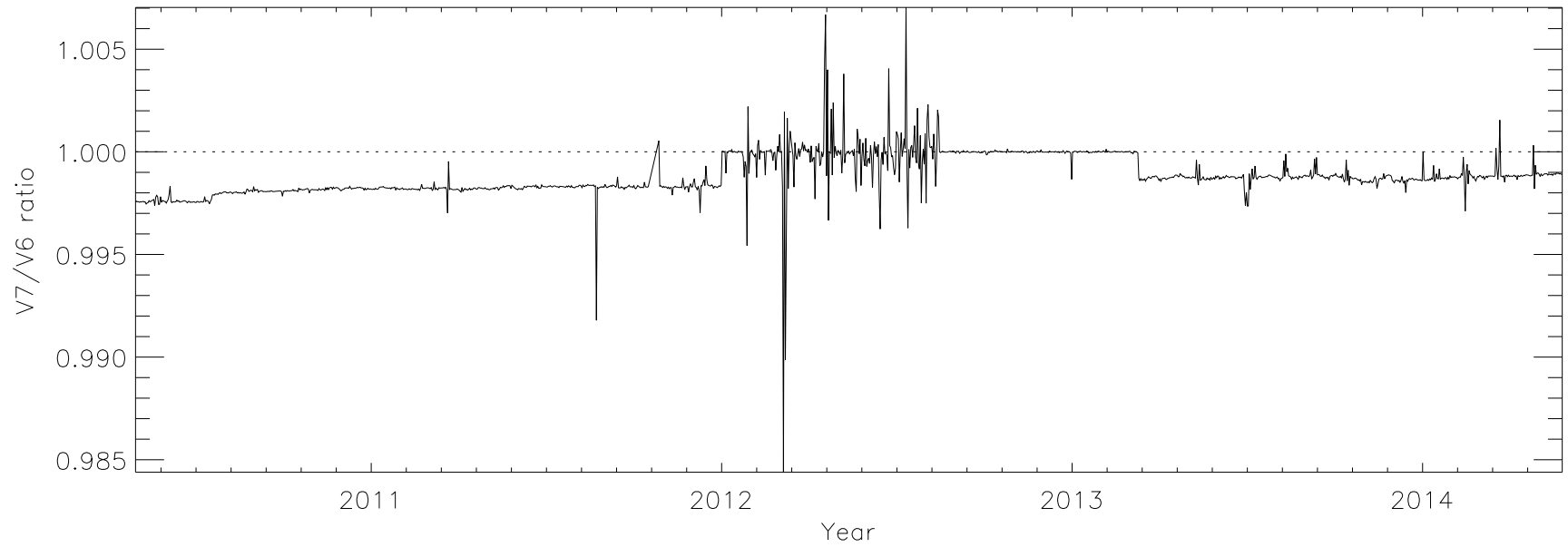
Fe IX 17.107
