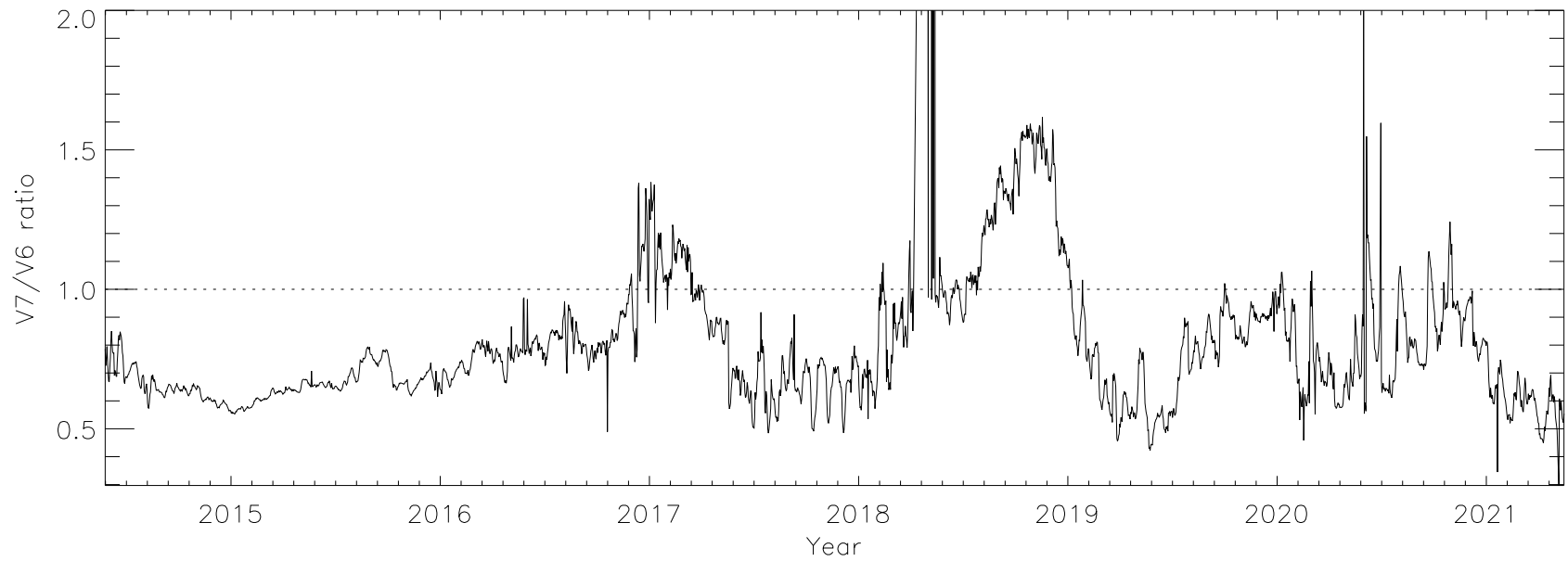
Fe XVI 36.076
