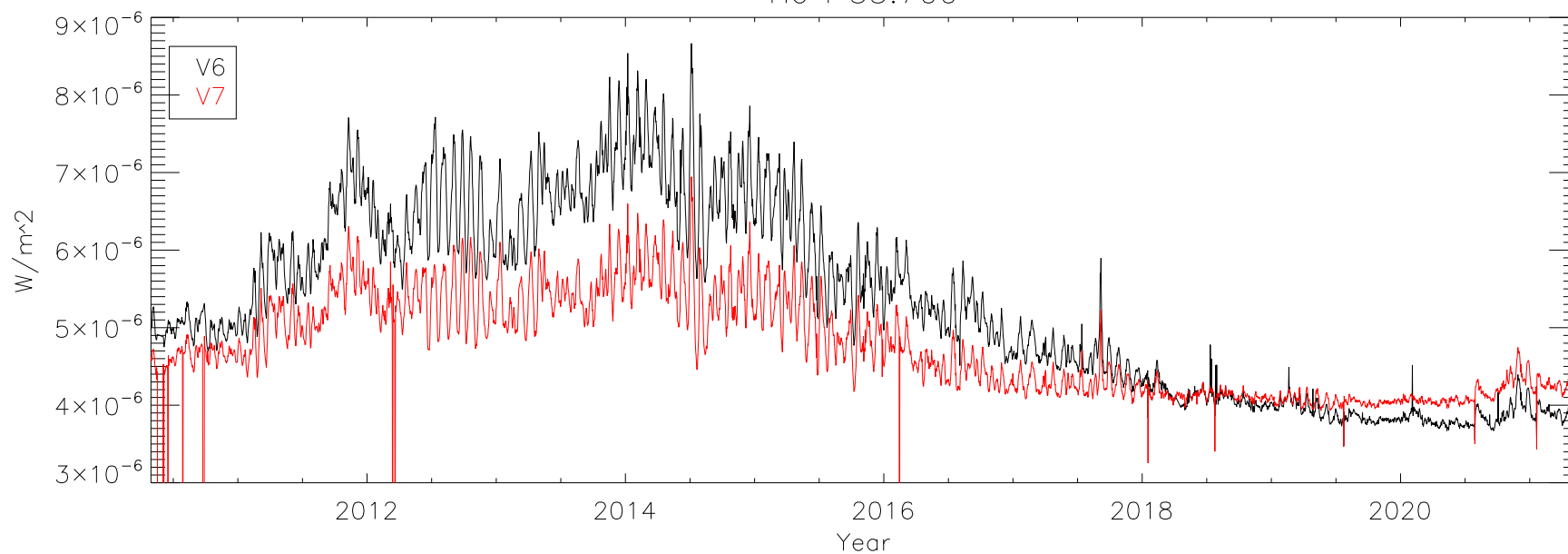
He I 53.700
