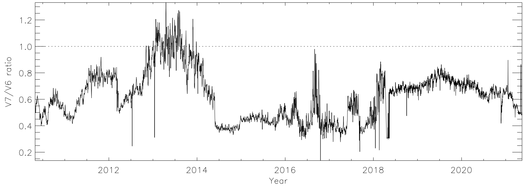
Fe XX 72.156
