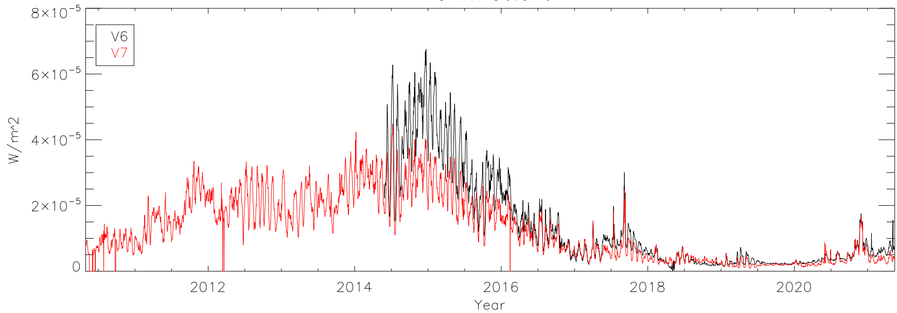
Fe XVI 36.076
