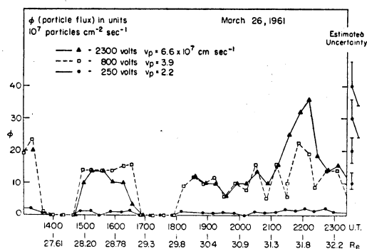
Fig. 4. Observed proton flux, 1300 to 2350 U.T., March 26, 1961.
