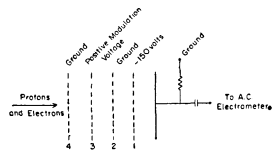
Fig. 1. Grid arrangement in cup.
