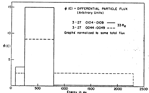
Fig. 7. Typical proton energy spectra.
