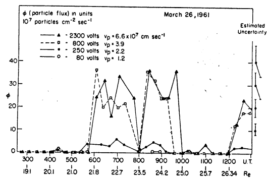
Fig. 3. Observed proton flux, 0300 to 1300 U.T., March 26, 1961.
