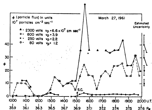
Fig. 6. Observed proton flux, 1000 to 2000 U.T., March 27, 1961.
