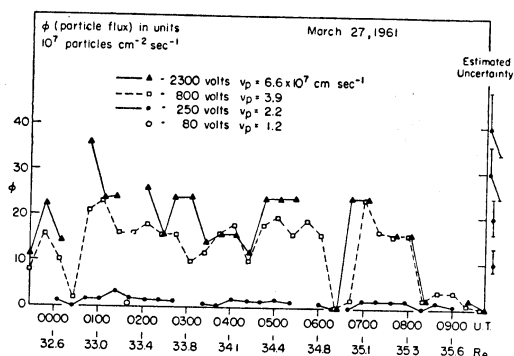
Fig. 5. Observed proton flux, 2350, U.T., March 26 to 1000 U.T., March 27, 1961.
