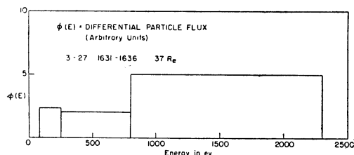
Fig. 8. Energy spectrum of protons, 1631-1636, U.T., March 27, 1961.
