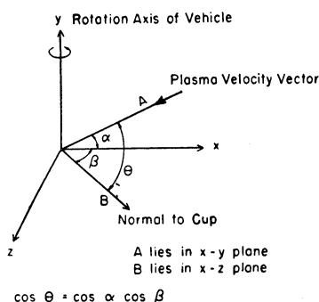
Fig. 9. Coordinate system showing \alpha , the minimum angle between the cup normal and the plasma velocity vector; \beta , the angular position of the cup normal in the x, z-plane; and \theta , the angle between the cup normal and the plasma velocity vector.
