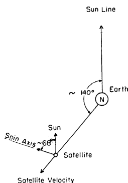
Fig. 2. Approximate spatial orientation of vehicle, looking down on the earth's north pole.
