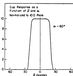
Fig. 10-14. Angular response curves of cup for different values of \alpha .
