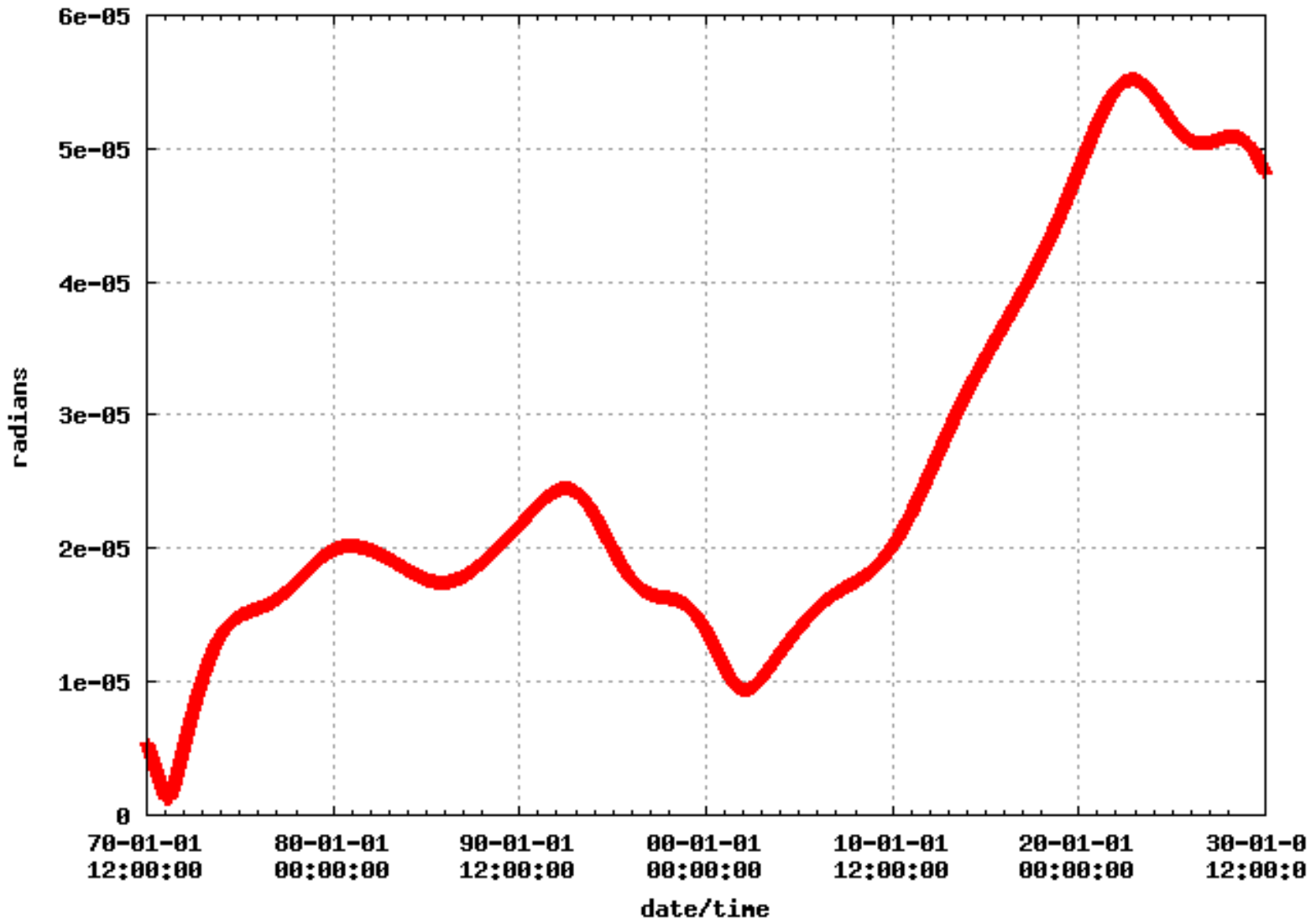
pck00010.tpc; IAU_JUPITER; total rotational difference with and w/o nut/prec terms
