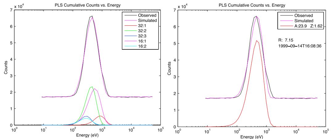
Figure A5. Fits for single species and multiple species—comparison suggests that ion temperature derived from fitting a single species over estimates the ion temperature by a factor of about 1.4.
