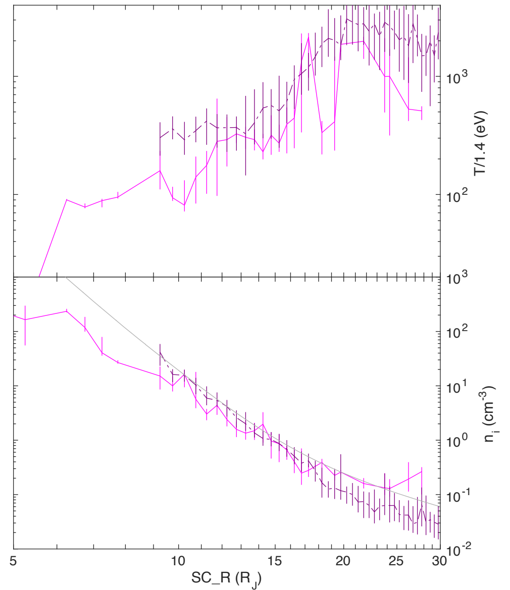
Dusk LT
