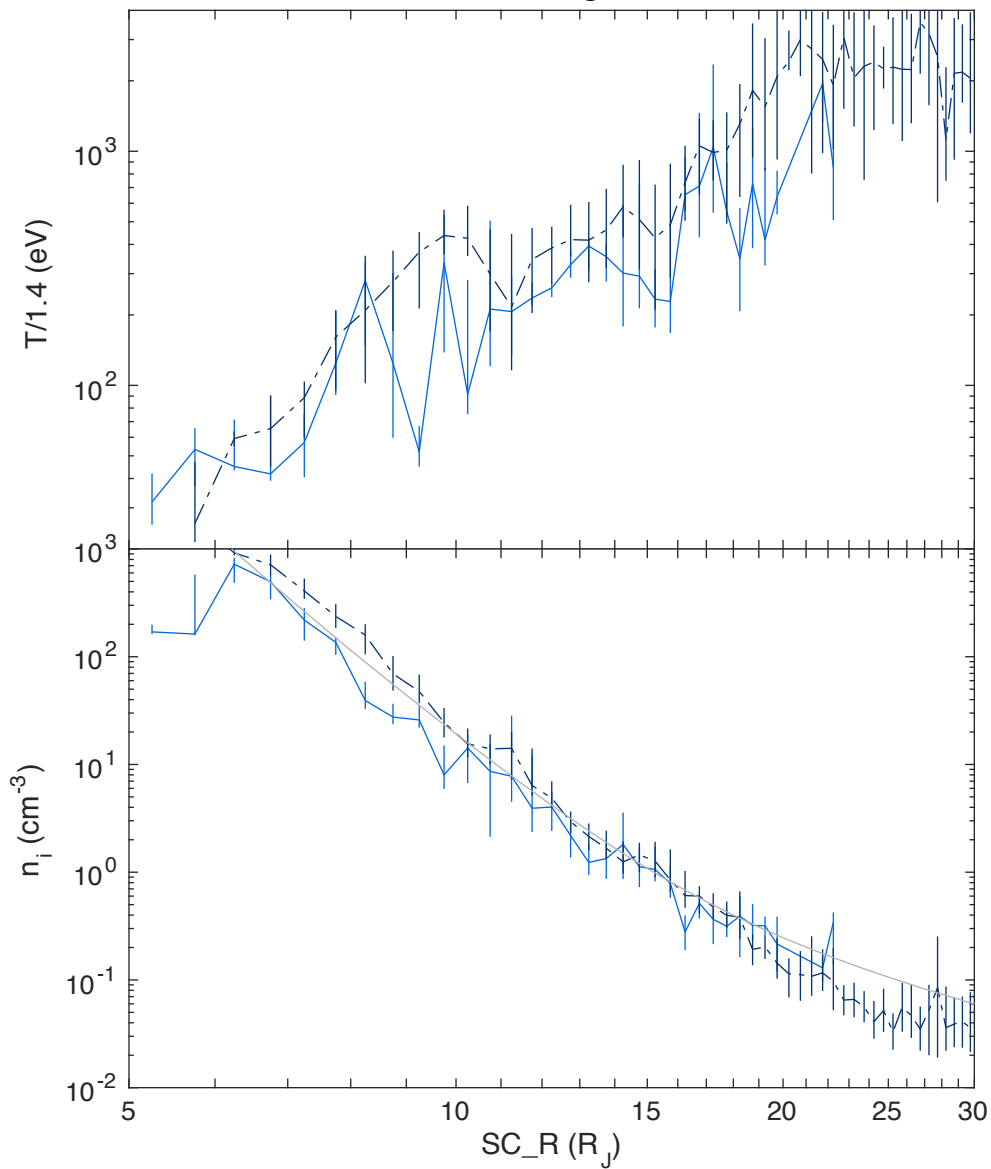
022 < E. Long. < 112
