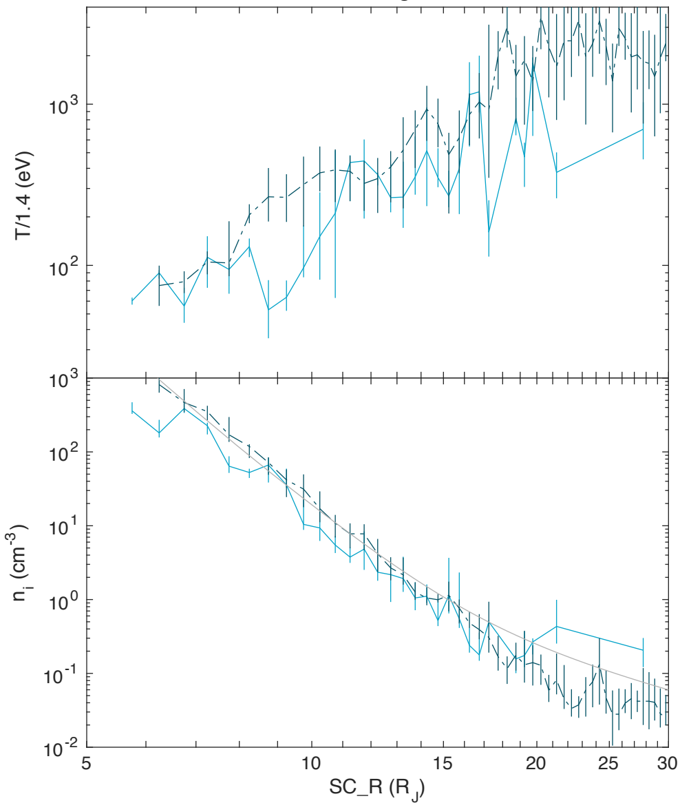
157 < E. Long. < 247
