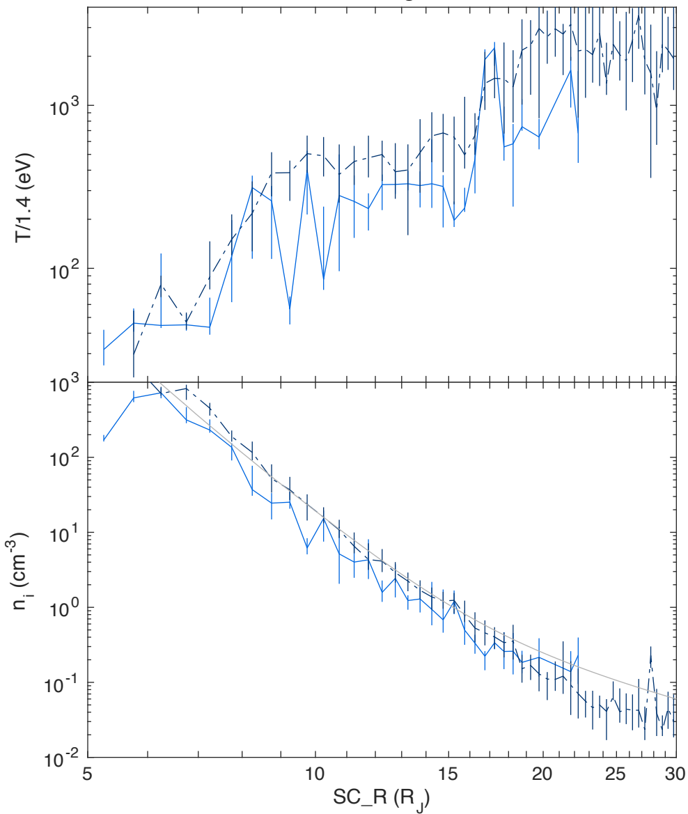
067 < E. Long. < 157
