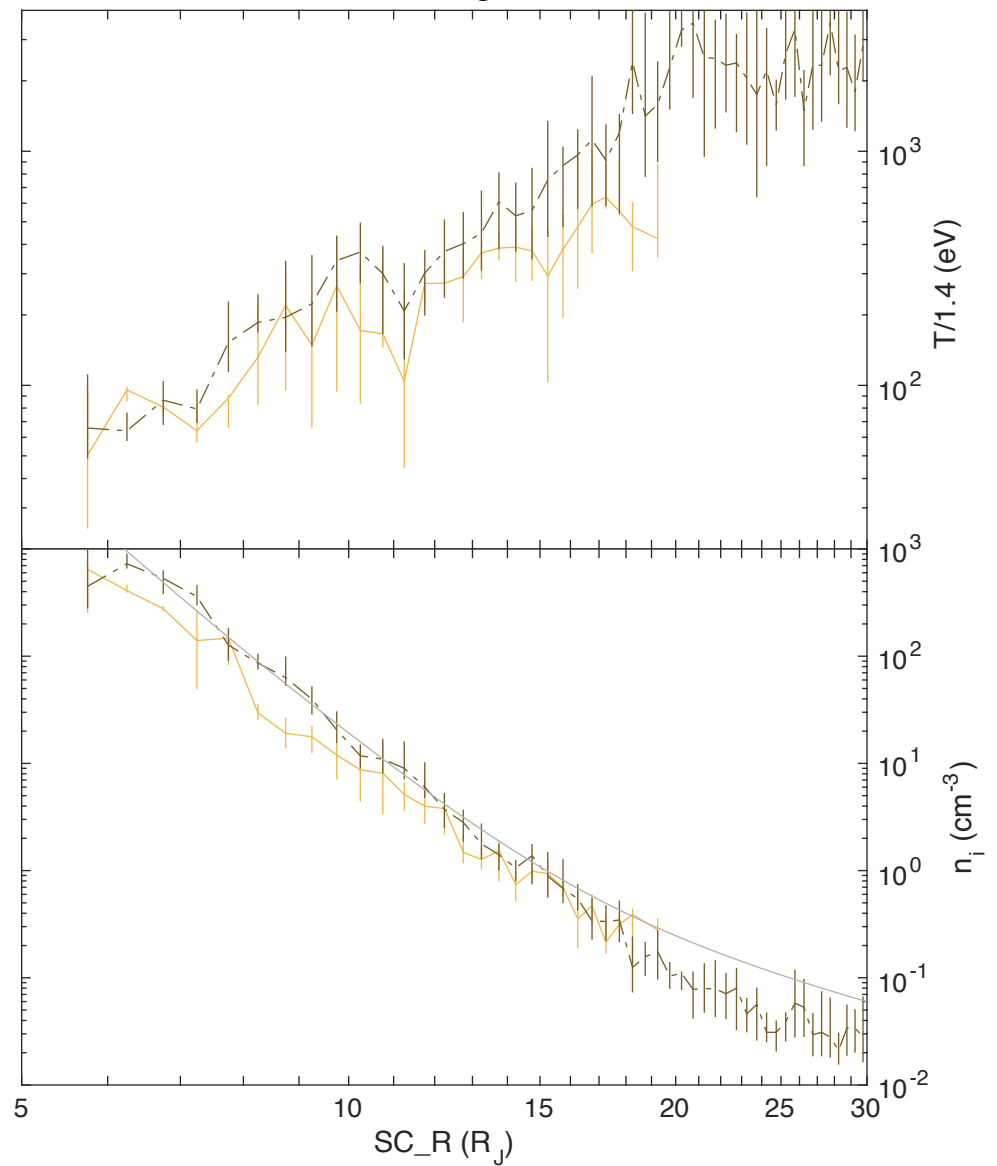
337 < E. Long. < 067
