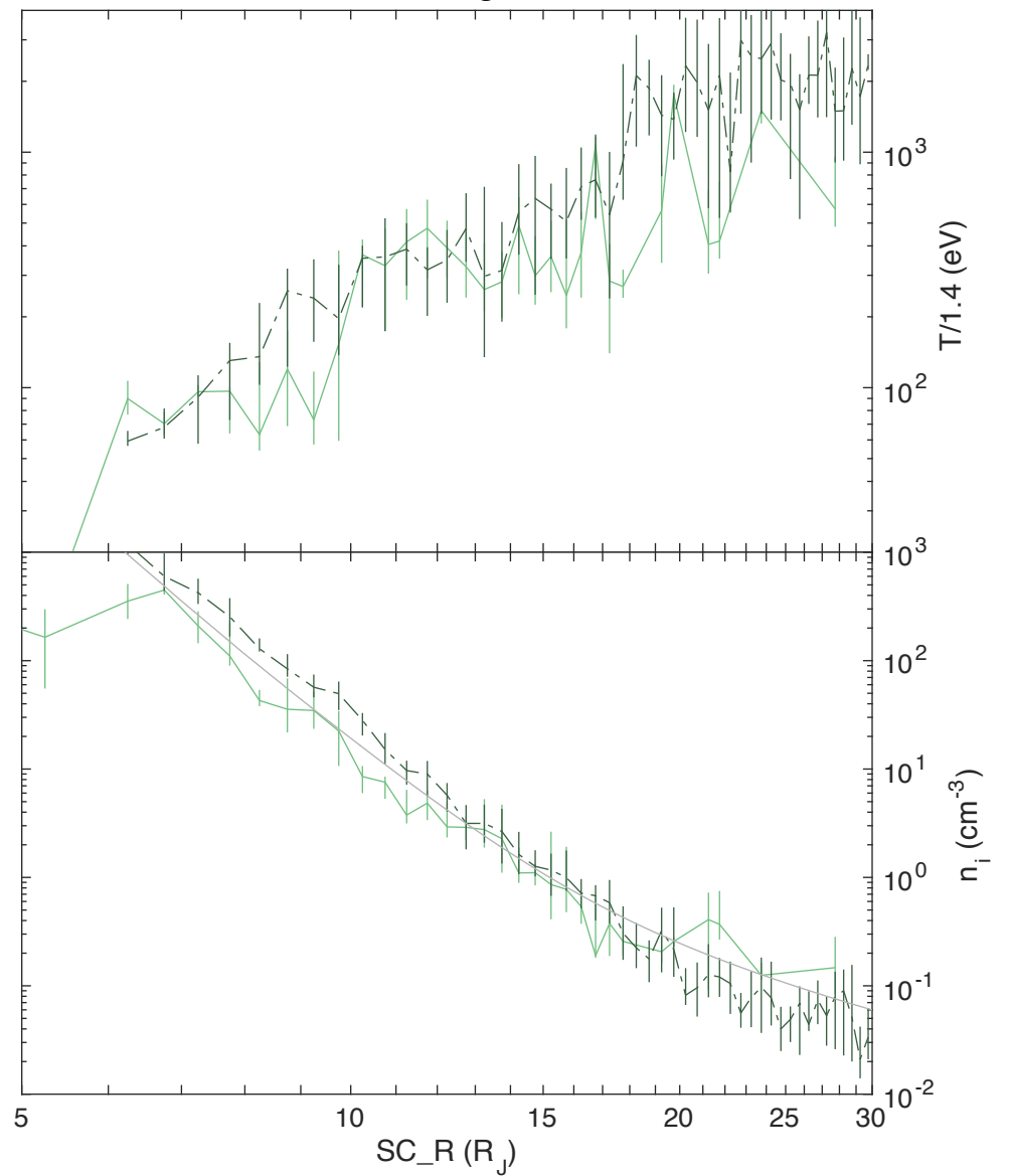
202 < E. Long. < 292
