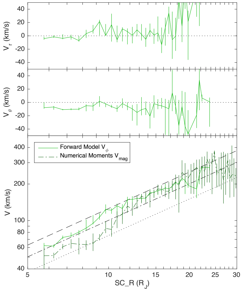
Dawn LT
