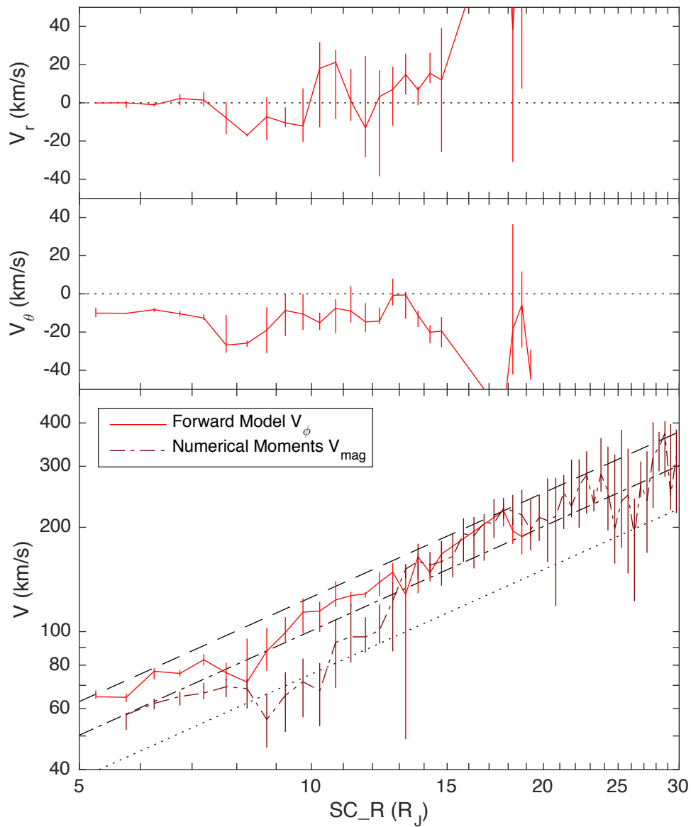
Noon LT
