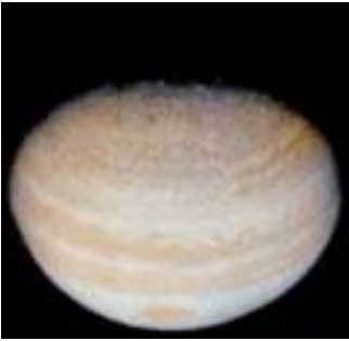
View of Jupiter taken by Pioneer 11
