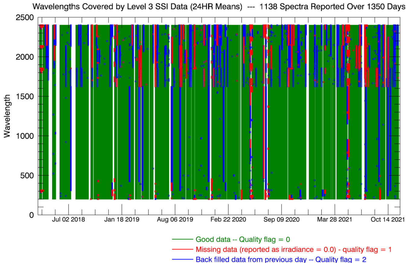
Figure 1: V07 TSIS-1 SIM data acquisition record. As of Dec. 12, 2021, the TSIS-1 SIM data are available on 84.3% of days since the beginning of nominal operations on March 14, 2018.
