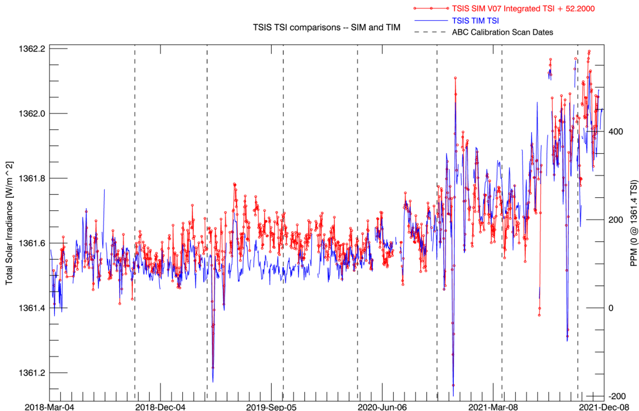
Figure 2: Comparison of V03 data release of TSIS-1 TIM (blue) Total Solar Irradiance (TSI) to the integrated Solar Spectral Irradiance (SSI) from the V07 data release of TSIS-1 SIM (red). An offset of +52.20 W m -2 has been added to the integrated SSI to account for bandpasses not measured by SIM.
